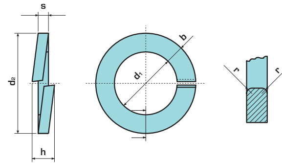
Lock washer with square end
